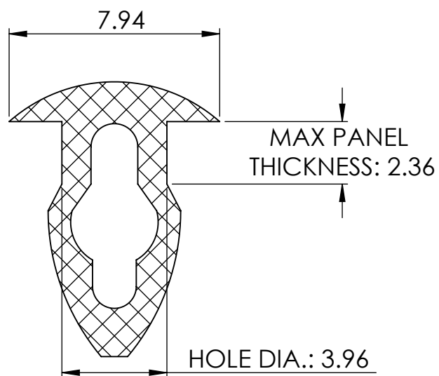
SECTION Y-Y
